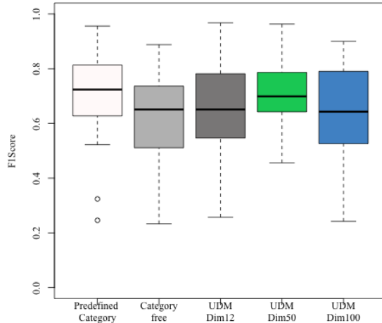
Figure 5: The comparison of the F1-score distribution of all tokens of the unified discriminative method vs. baselines (leftmost two bars). Minimum, mean, and maximum F1-score performance of UDM using 50 latent dimensions is both high and consistent compared to both baselines and other latent dimension variants.
