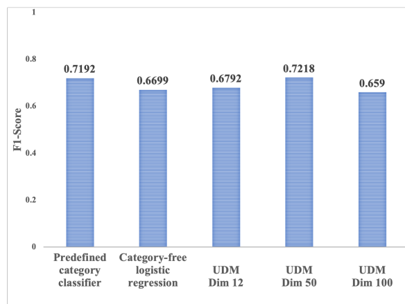
Figure 6: Averaged micro F1-score performance of visual classifiers. The unified discriminative method (UDM) shows improved performance than predefined category classifier where classifiers are learned per category and the category-free logistic regression where the concatenated feature set is learned per word.
