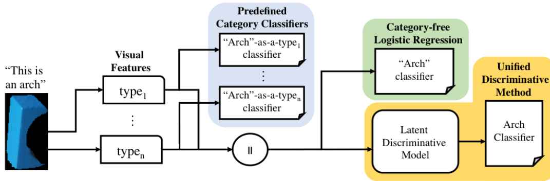
Figure 4: Diagram of approaches. The predefined category classifier—a current approach in the literature—learns one visual classifier for every visual category, accepting input from the respective visual characteristics (blue box). Category-free logistic regression is a baseline that learns a single classifier for each word, accepting cumulative visual features as input (green box). On the far right (yellow box), the Unified Discriminative Method—described in this paper—generates visual classifiers for each word, accepting latent visual embedding generated from cumulative visual features as input.
