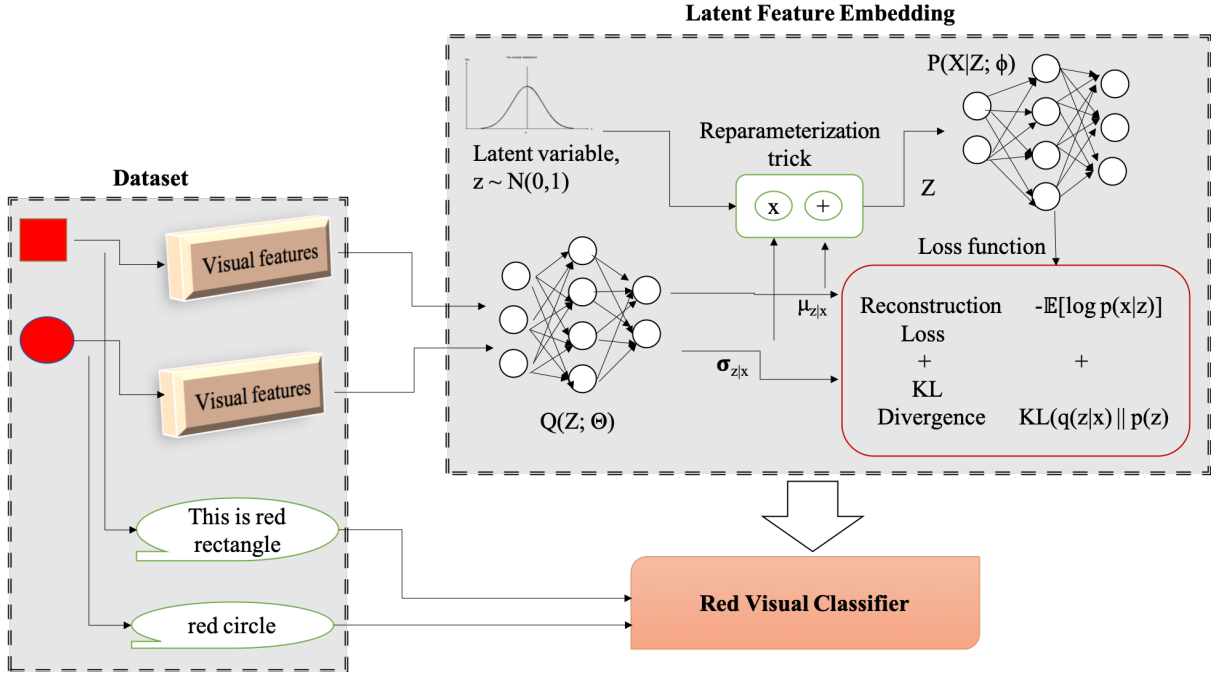
Figure 1: Design diagram of the unified discriminative method. For every object, all kinds of features are extracted and learn it through a latent feature generative model to generate a representative embedding of the feature vector. The extracted embedding is joined with a visual classifier denoted by the “language term.”
